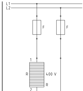
Illustration 11: Wiring diagram without thermostat - 400 V
