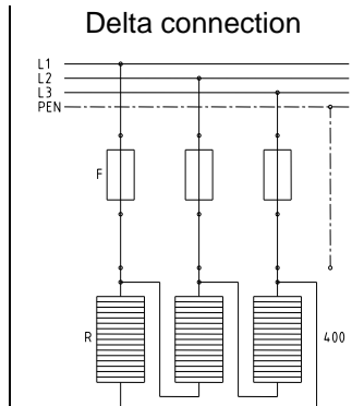
Illustration 15: Wiring diagram with thermostat - 400 V Δ
