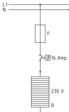
Illustration 8: Wiring diagram with thermostat - 230 V
