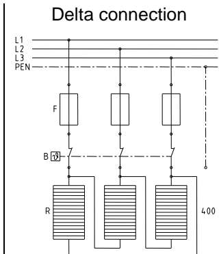
Illustration 14: Wiring diagram with thermostat - 400 V Δ
