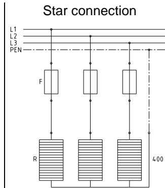
Illustration 13: Wiring diagram with thermostat - 400 V ⋄
