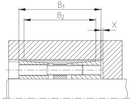
Illustration 4: Space for disassembly
