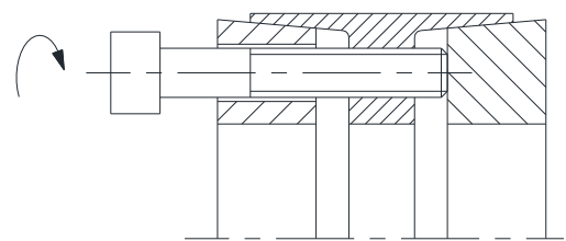
Illustration 7: Fastening the rear pressure ring
