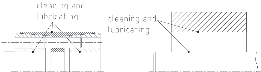
Illustration 5: Cleaning and lubricating the surfaces
