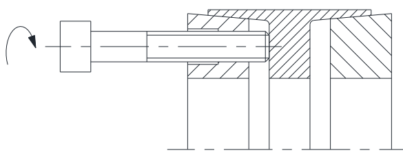
Illustration 6: Fastening the front pressure ring
