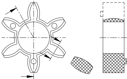
Illustration 9: ROTEX® spider
