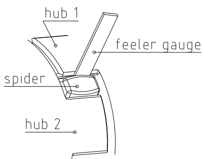
Illustration 10: Inspection of the limit of wear
