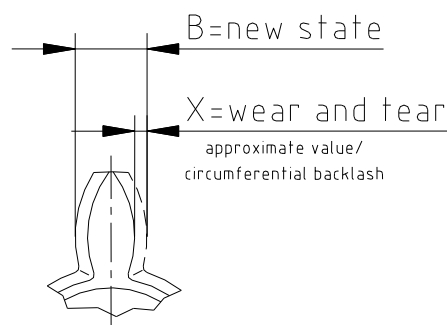
Illustration 11: Wear of spider
