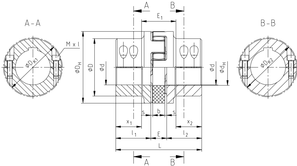
Illustration 2: ROTEX®, type A-H (material: EN-GJS-400-15)
