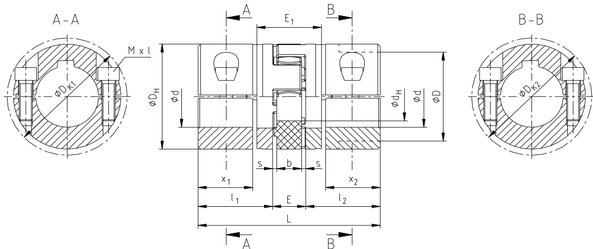
Illustration 1: ROTEX®, type A-H (material: steel)
