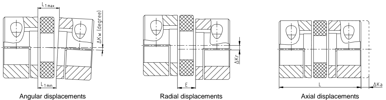
Illustration 6: Displacements
