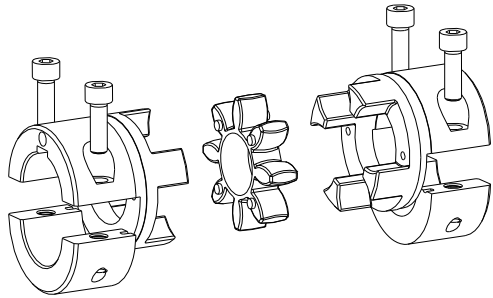
Illustration 8: ROTEX®, type A-H
