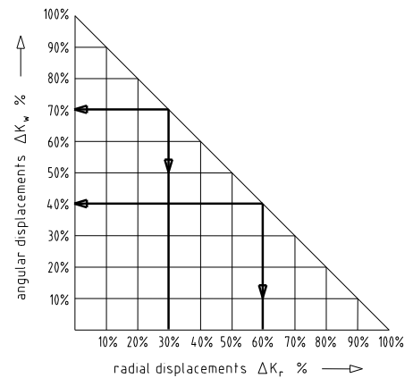
Illustration 7: Combinations of displacement
