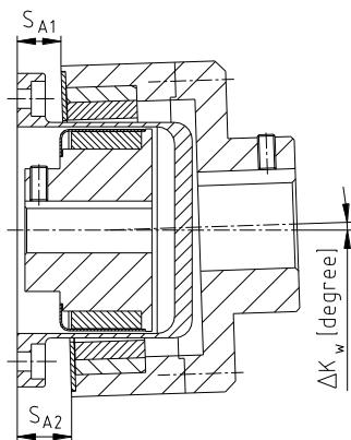
Angular displacement
