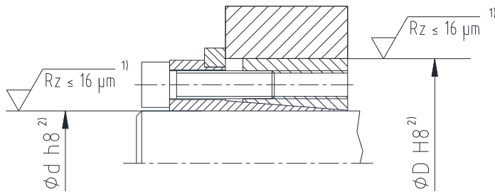
Illustration 3: Tolerances and surfaces (example: CLAMPEX® KTR 201)
