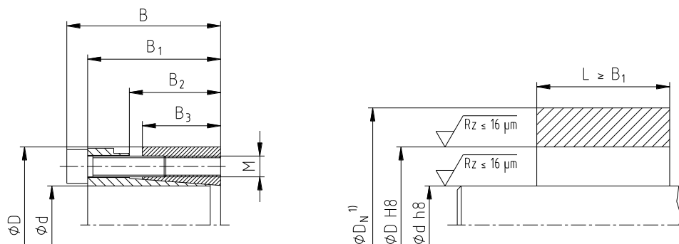
Illustration 1: CLAMPEX® KTR 200
