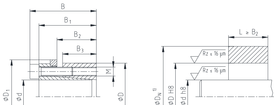
Illustration 2: CLAMPEX® KTR 201
