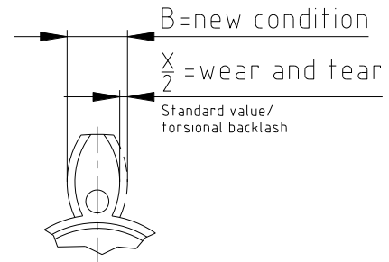
Illustration 11: Wear of spider
