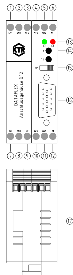
Illustration 13: Connection housing DF2
