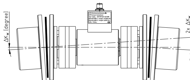
Angular displacement
