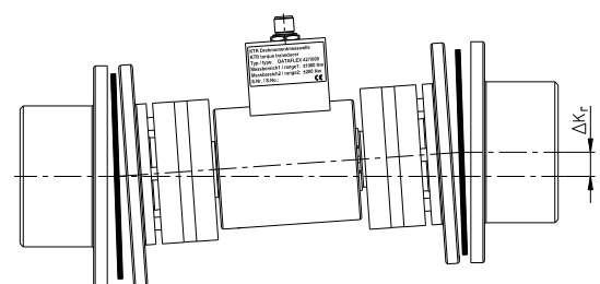
Radial displacement
