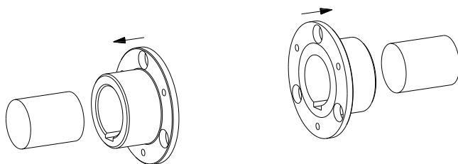
Illustration 9: Assembly of the hubs on the driving and driven side
