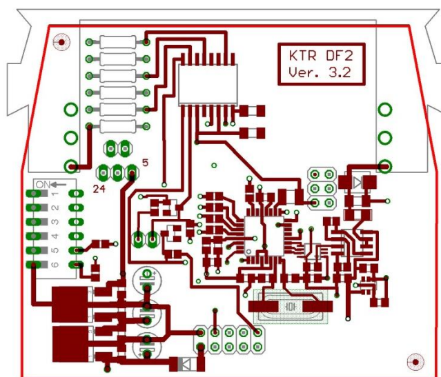
Illustration 20: Modification of voltage level for the speed signal/direction signal
