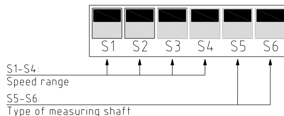
Illustration 21: Switch positions
