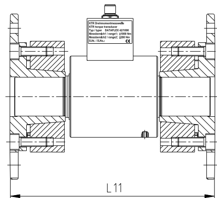
Illustration 8: Alignment to dimension L11
