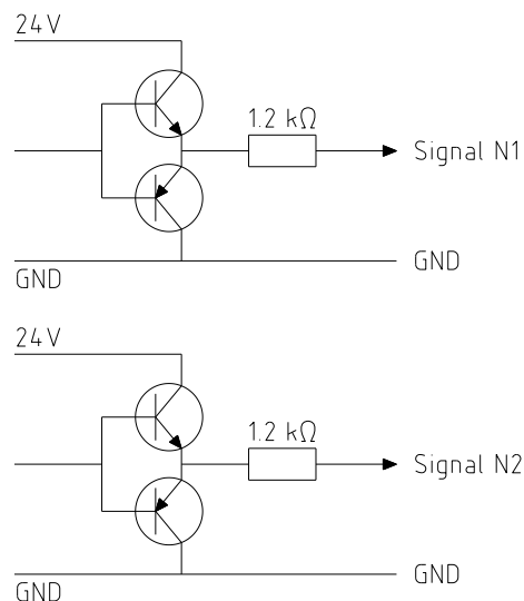
Illustration 19: Output circuit of speed outputs
