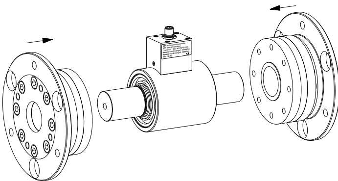
Illustration 7: Assembly of clamping ring hubs
