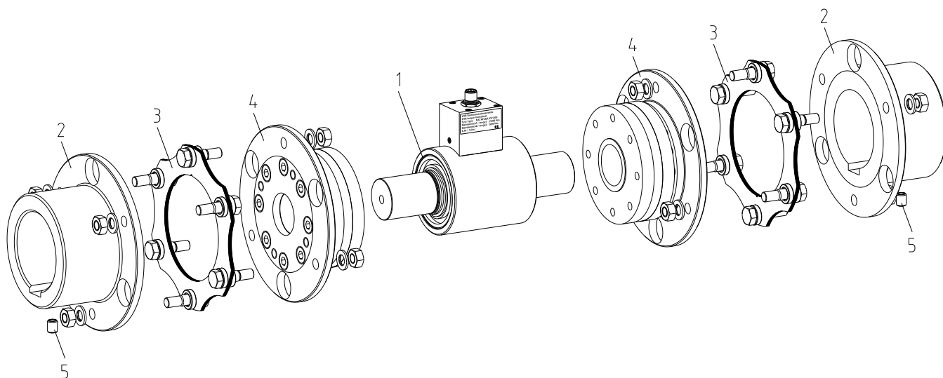
Illustration 3: DATAFLEX® 42 torque measuring shaft with RADEX®-N
