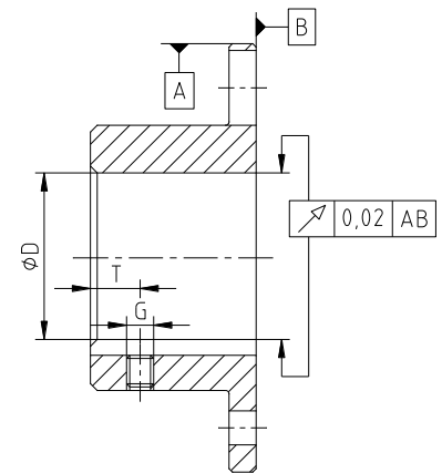
Illustration 4: Concentricity and axial runout
