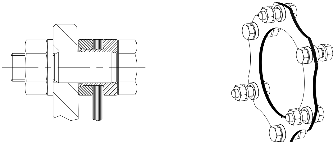
Illustration 11: Assembly of the laminae sets
