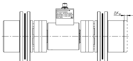
Axial displacement
