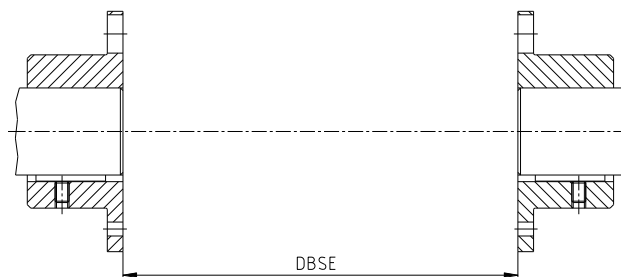
Illustration 10: Alignment to dimension DBSE
